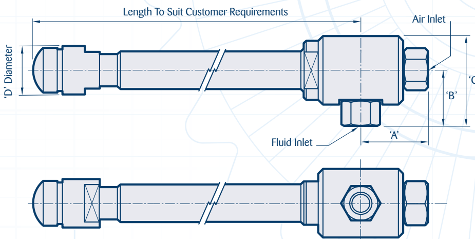
Round Version Nozzle Assembly Dimensions (inches/mm)
